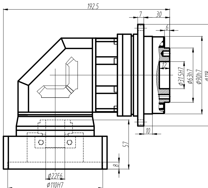
标准轴 Standard output shaft
